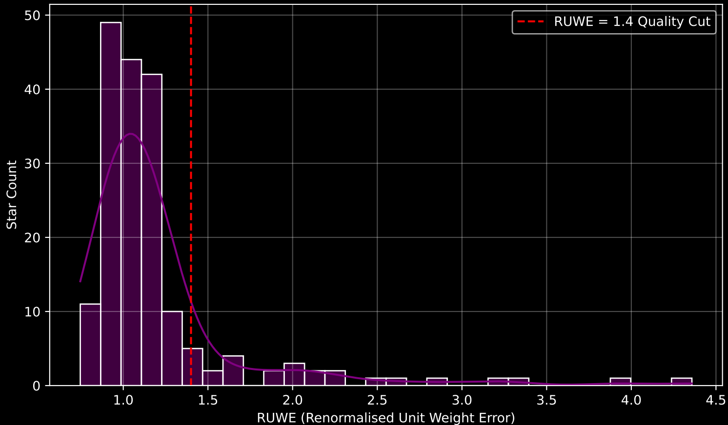
GAPOGEE DR17 Field [CVZTILE_101+39_btx] RUWE Distribution (n= 183)
