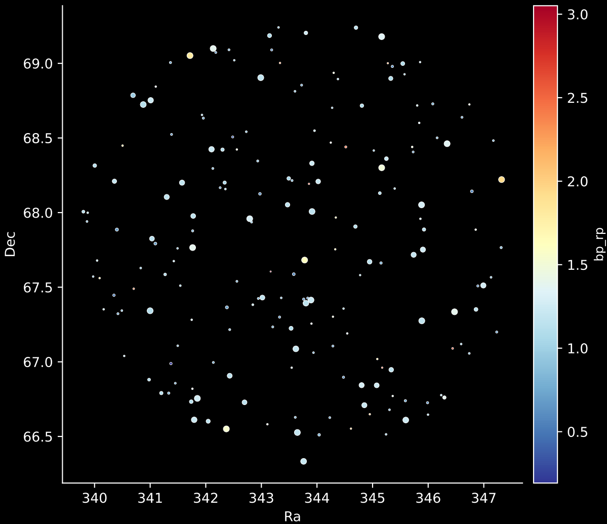
APOGEE DR17 Field: [CVZTILE_101+39_btx] Stars: 190
