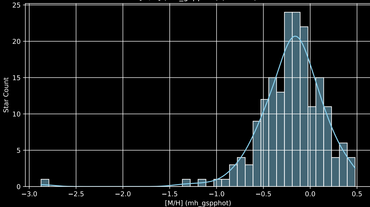
APOGEE DR17 Field: [CVZTILE_101+39_btx [M/H] (mh_gspphot) (n= 185)
