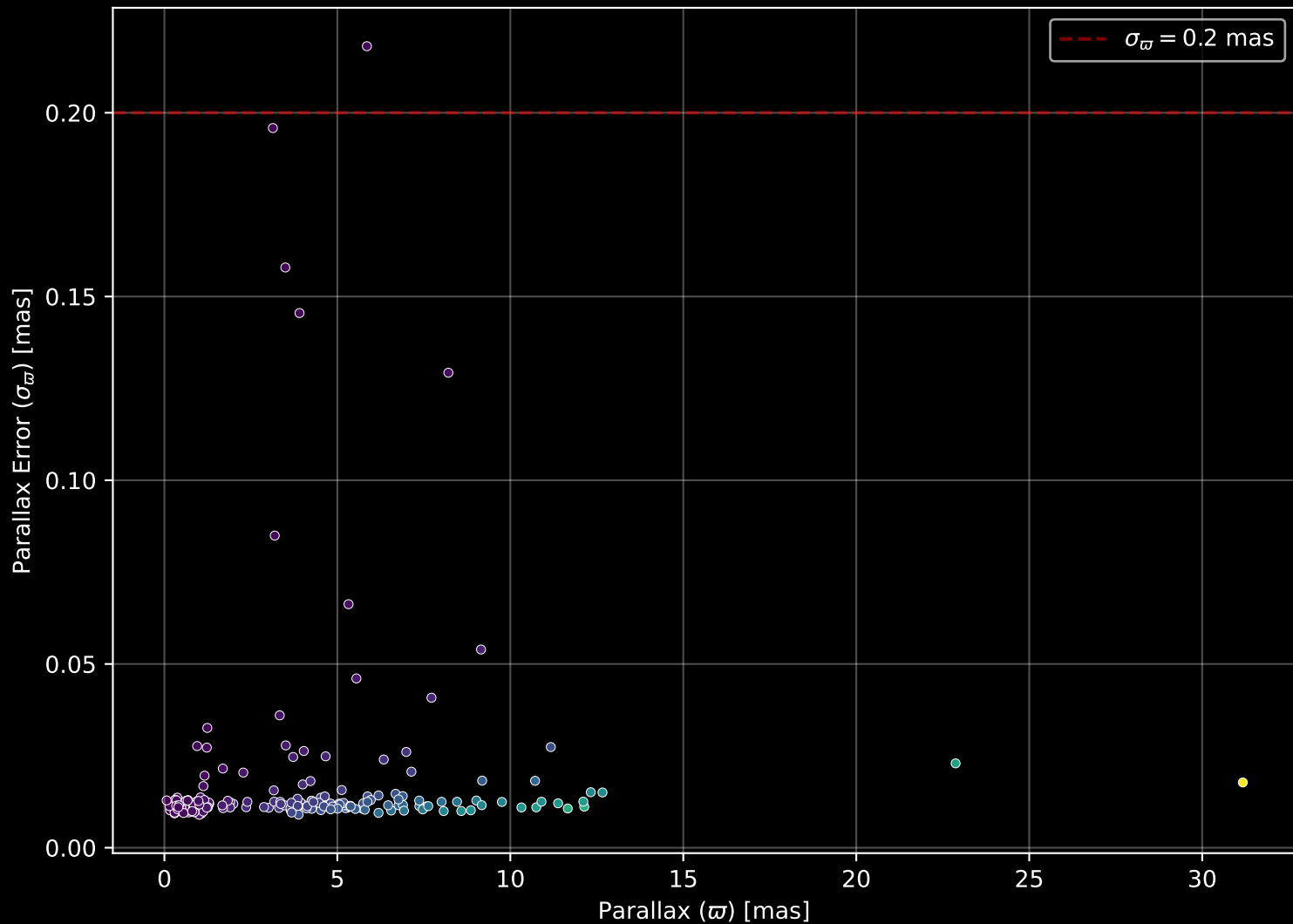
APOGEE DR17 Field: [CVZTILE_101+39_btx] Parallax Quality (n= 190)
