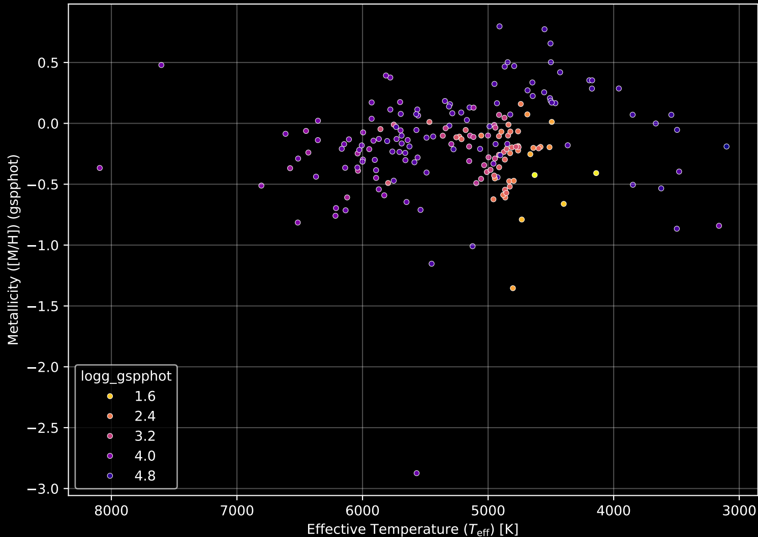
APOGEE DR17 Field: [CVZTILE_101+39_btx] Stellar Population Parameters (n= 190)
