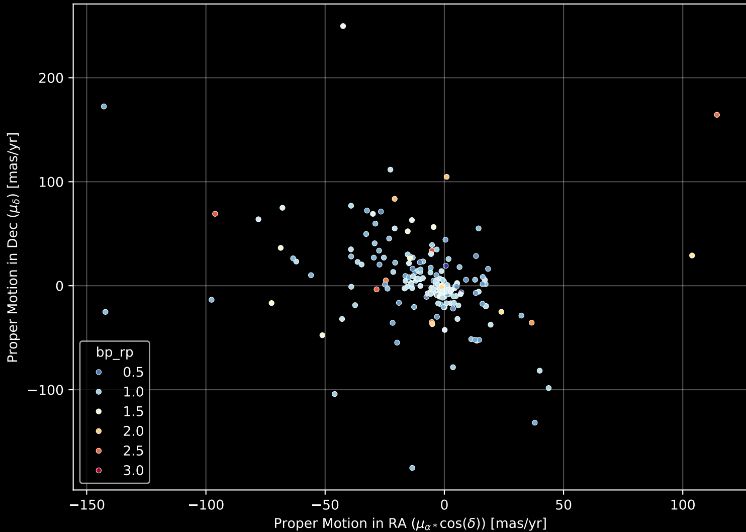
APOGEE DR17 Field: [CVZTILE_101+39_btx] Proper Motion Diagram (n= 190)
