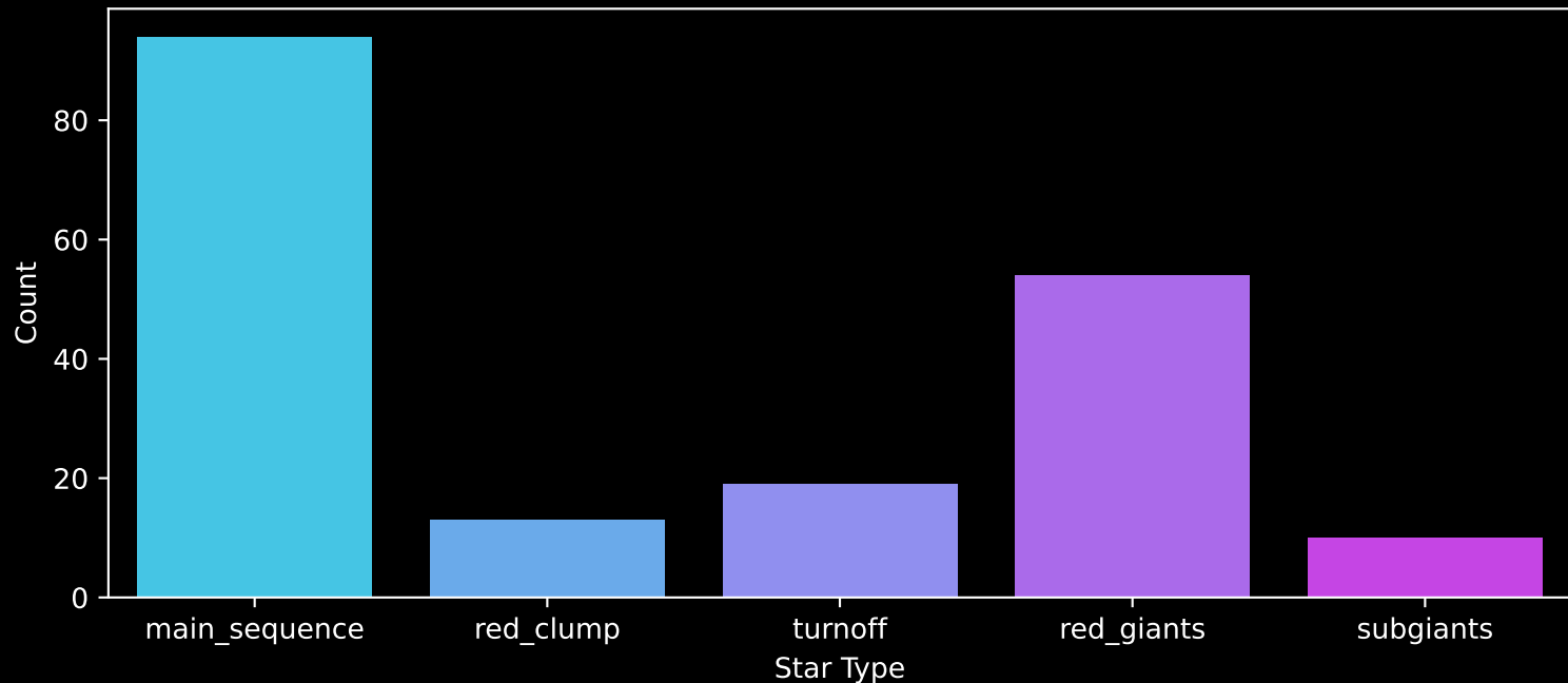
APOGEE DR17 Field: [CVZTILE_101+39_btx] Count plot of Star Type
